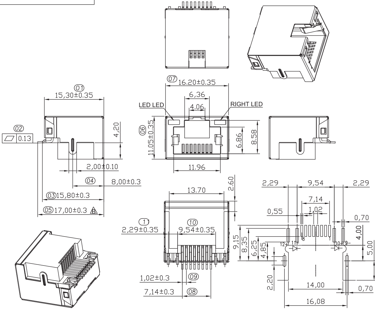
PCBLAYOUT TOP VIEW TOL:±0.05
